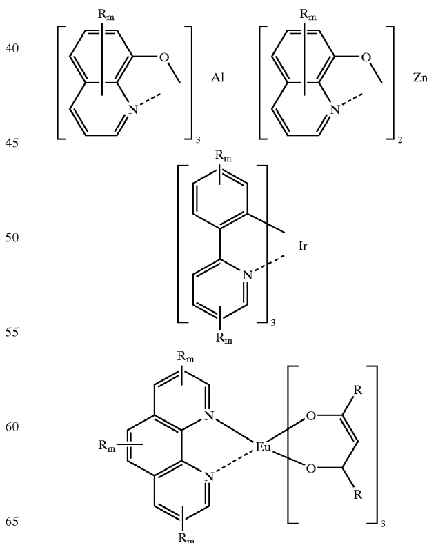
Scheme 4. Metal complexed organo-metallic compounds.
