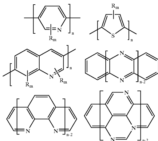
Scheme 3. Heterocyclic/fused ring heterocyclic combinations.
